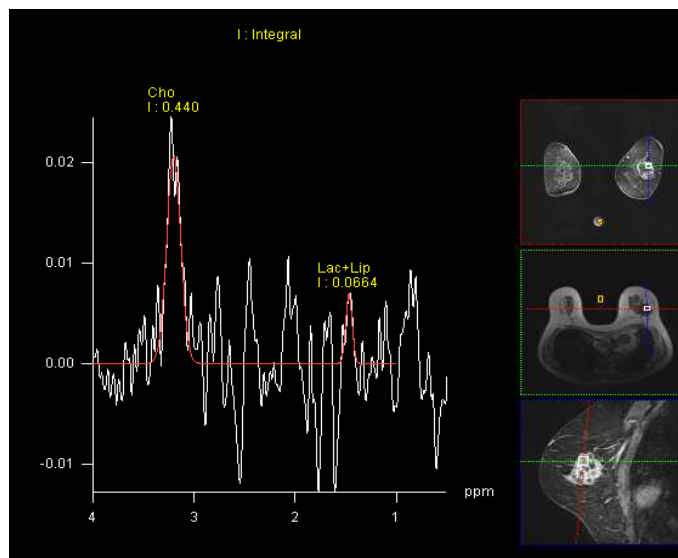
乳腺 MRS
